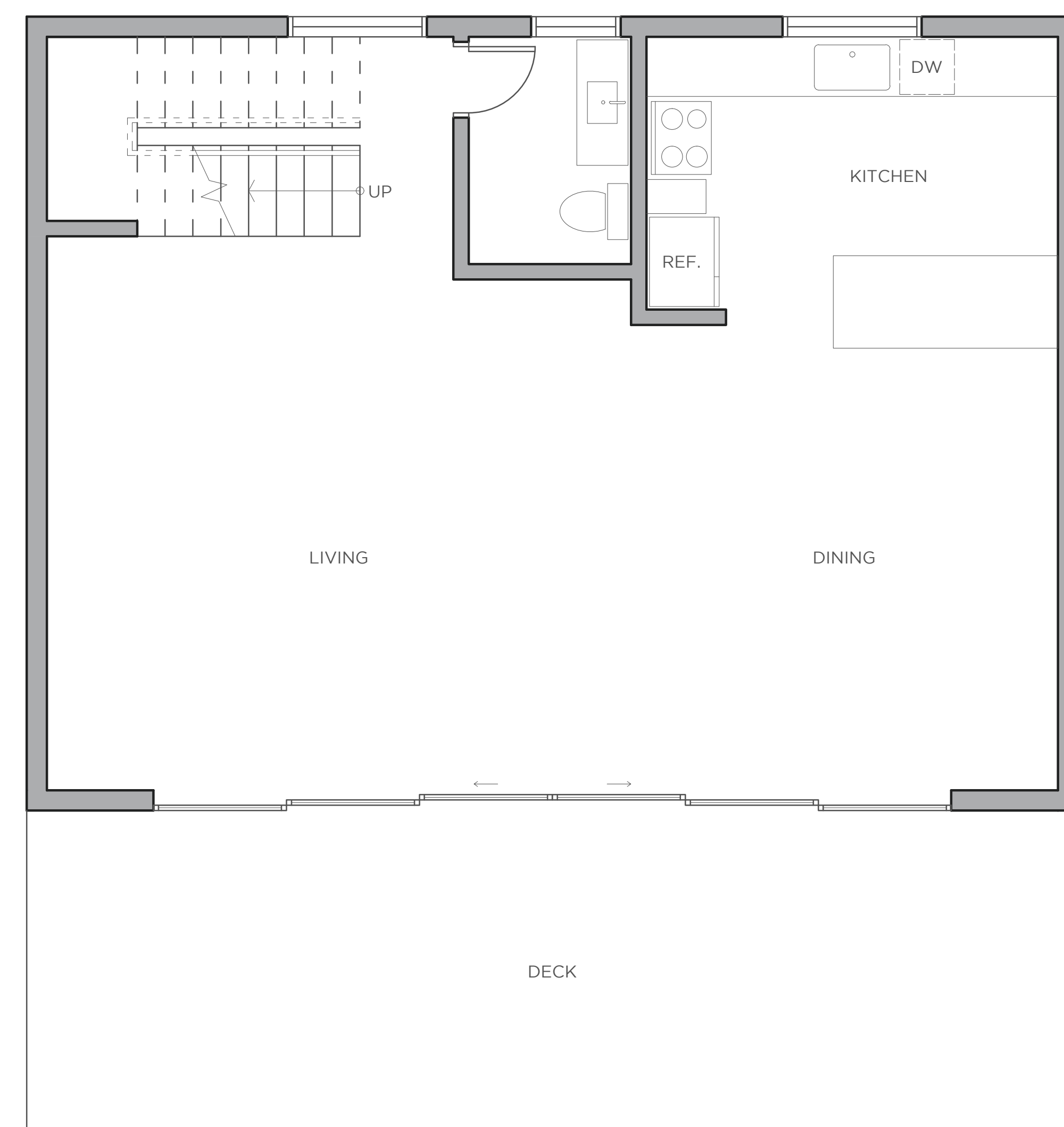
SECOND FLOOR
